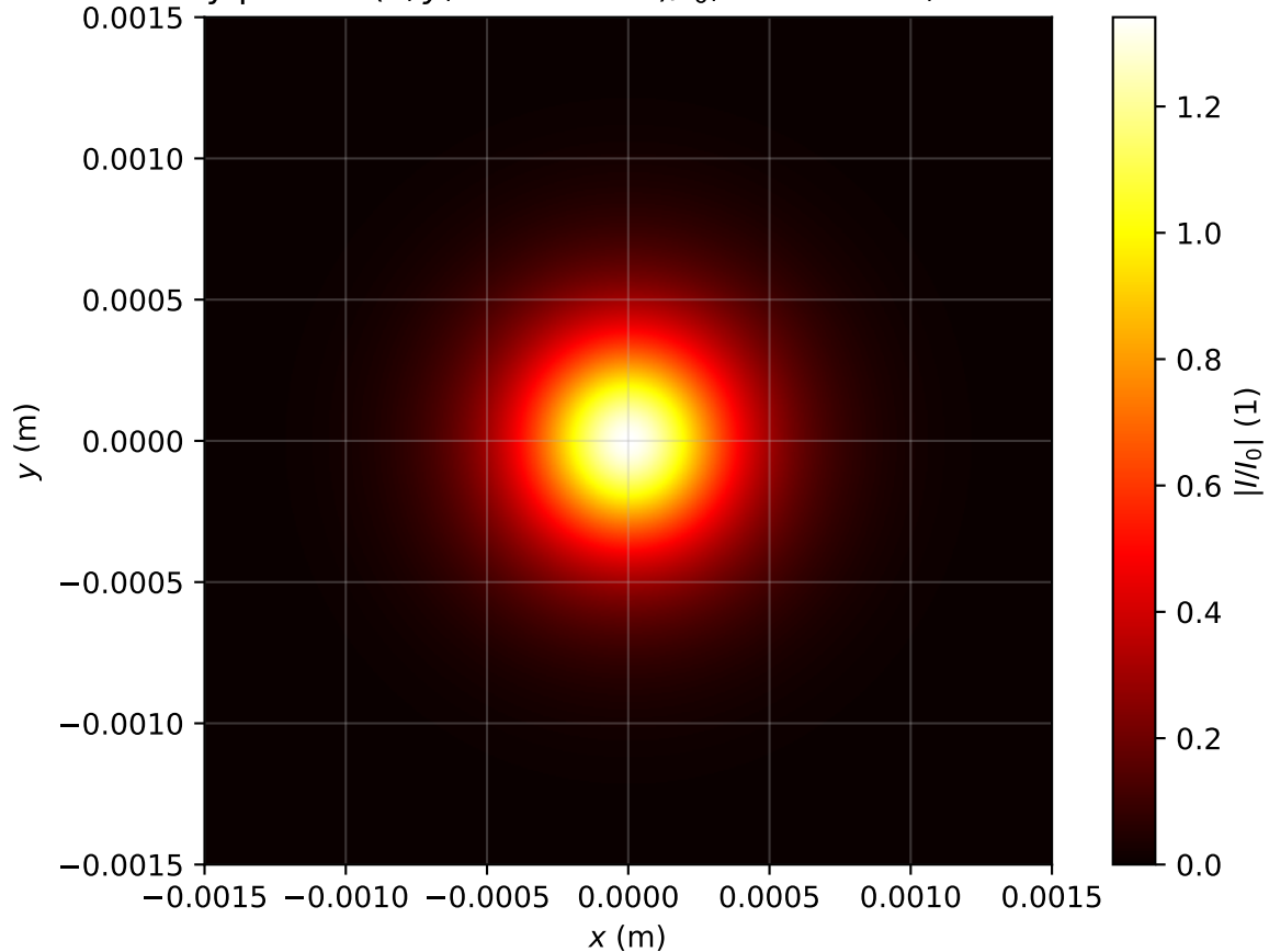
Intensity profile I(x, y, z = 0.876m)/I_0 , Pin=0.9Pcr, artificial time
